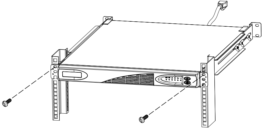
Figure 10. Securing the UPS in a 19" Rack
